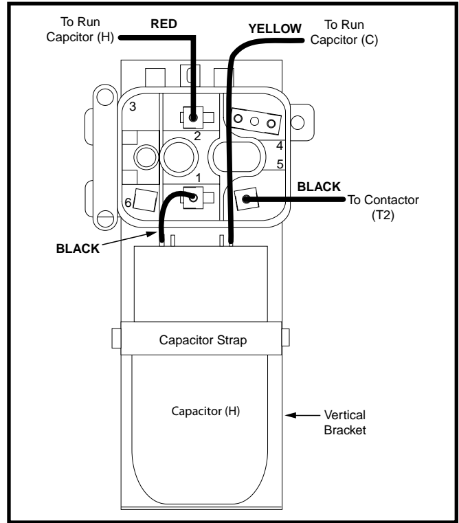
Figure 2. Vertical Bracket Installation
