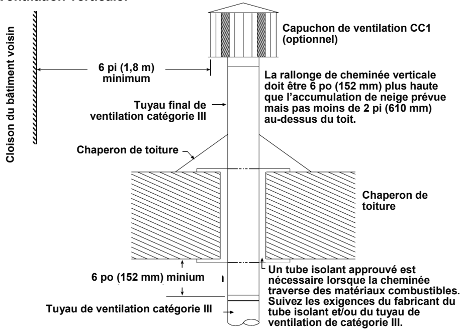
Figure 7.a Ventilation verticale.
