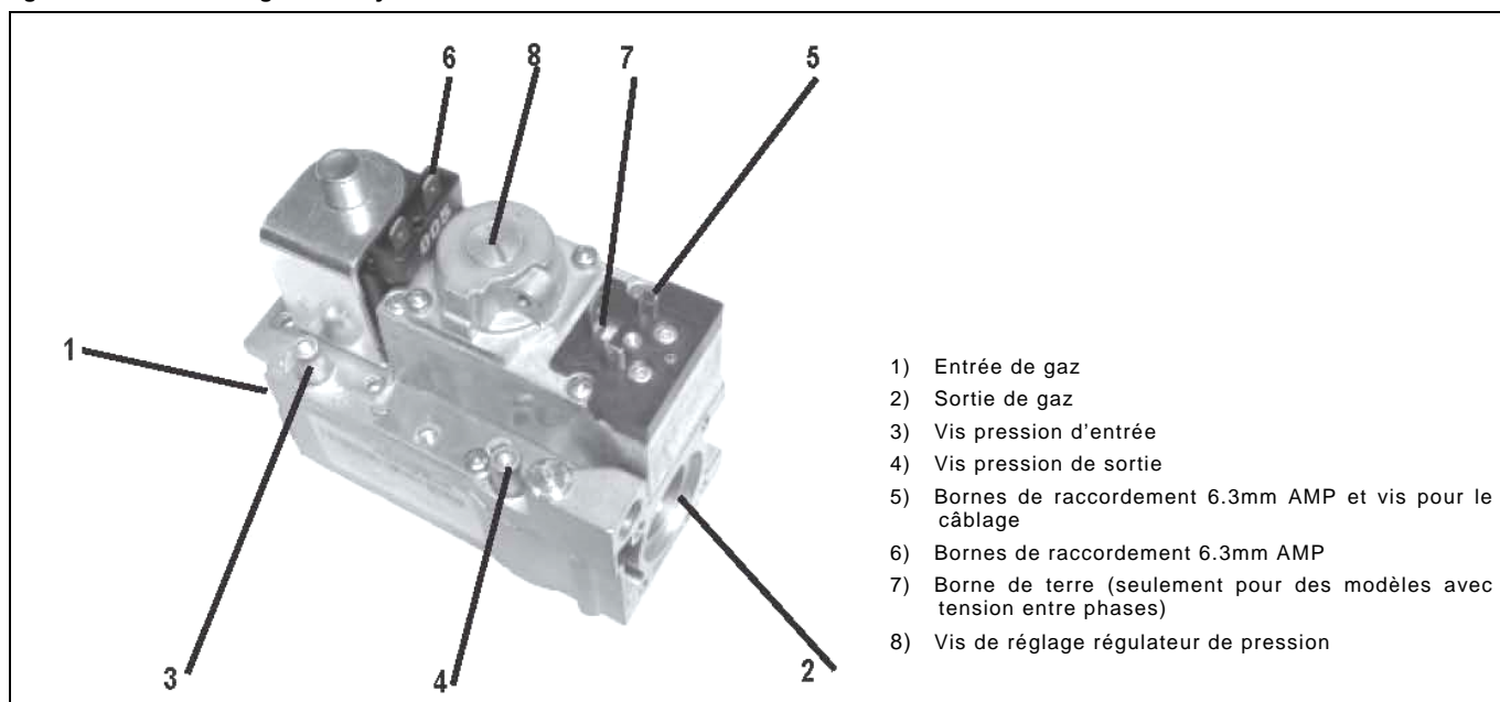
Figure 12: Vanne de gaz Honeywell
